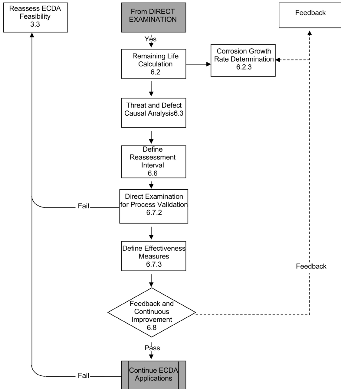
Figure 7: Postassessment Step (Numbers refer to paragraphs in this standard.)
