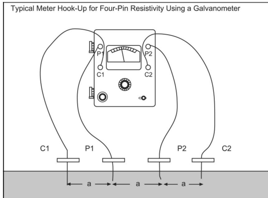
Figure A2: Four-Pin Method with Galvanometer
