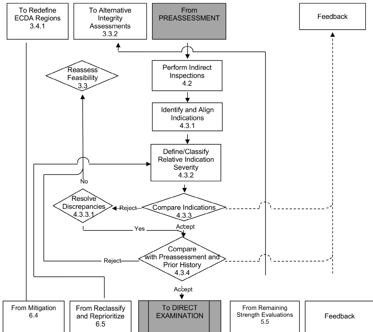
Figure 5: Indirect Inspection Step (Numbers refer to paragraphs in this standard.)
