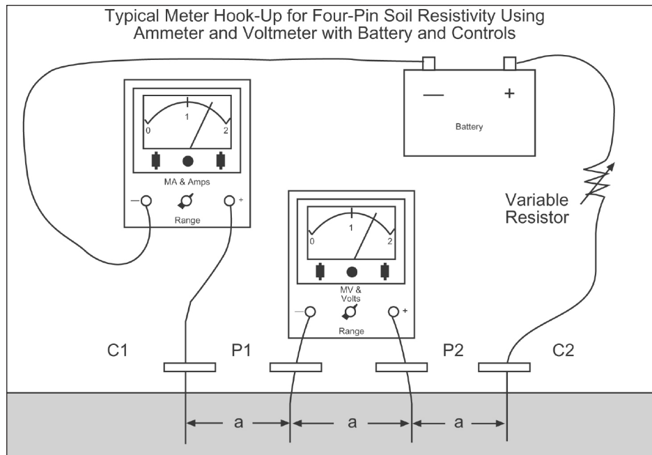
Figure A1: Four-Pin Method with Voltmeter and Ammeter
