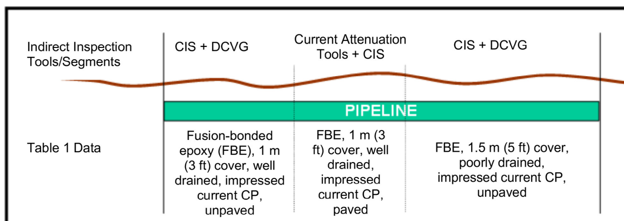
Figure 4: Example Selection of Indirect Inspection Tools
