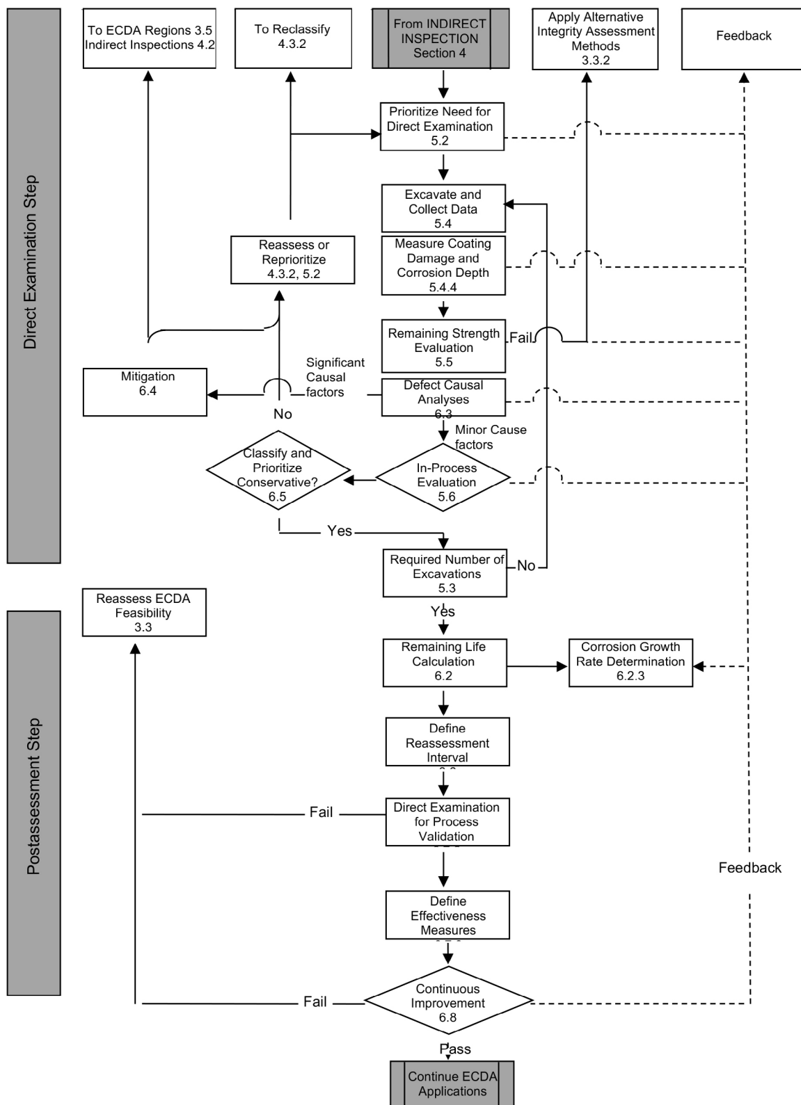
Figure 1(b): External Corrosion Direct Assessment Flow Chart—Part 2 (Numbers refer to paragraphs in this standard.)
